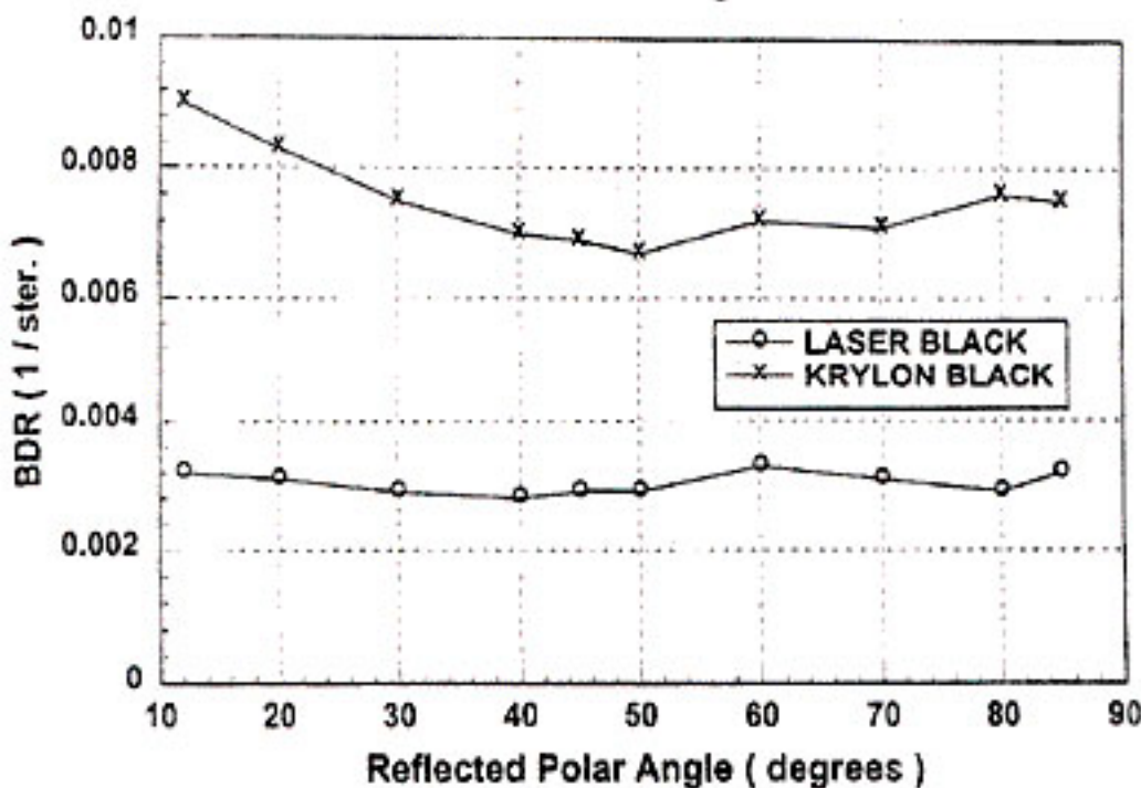
BRDF at 0.54 \mu\text{m} , 0 Degrees Incidence
