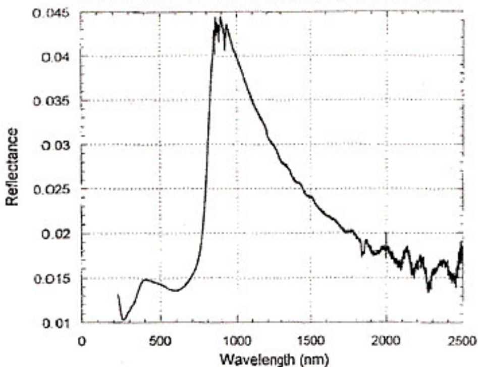
Total Reflectance of Laser Black on Thick Substrate
